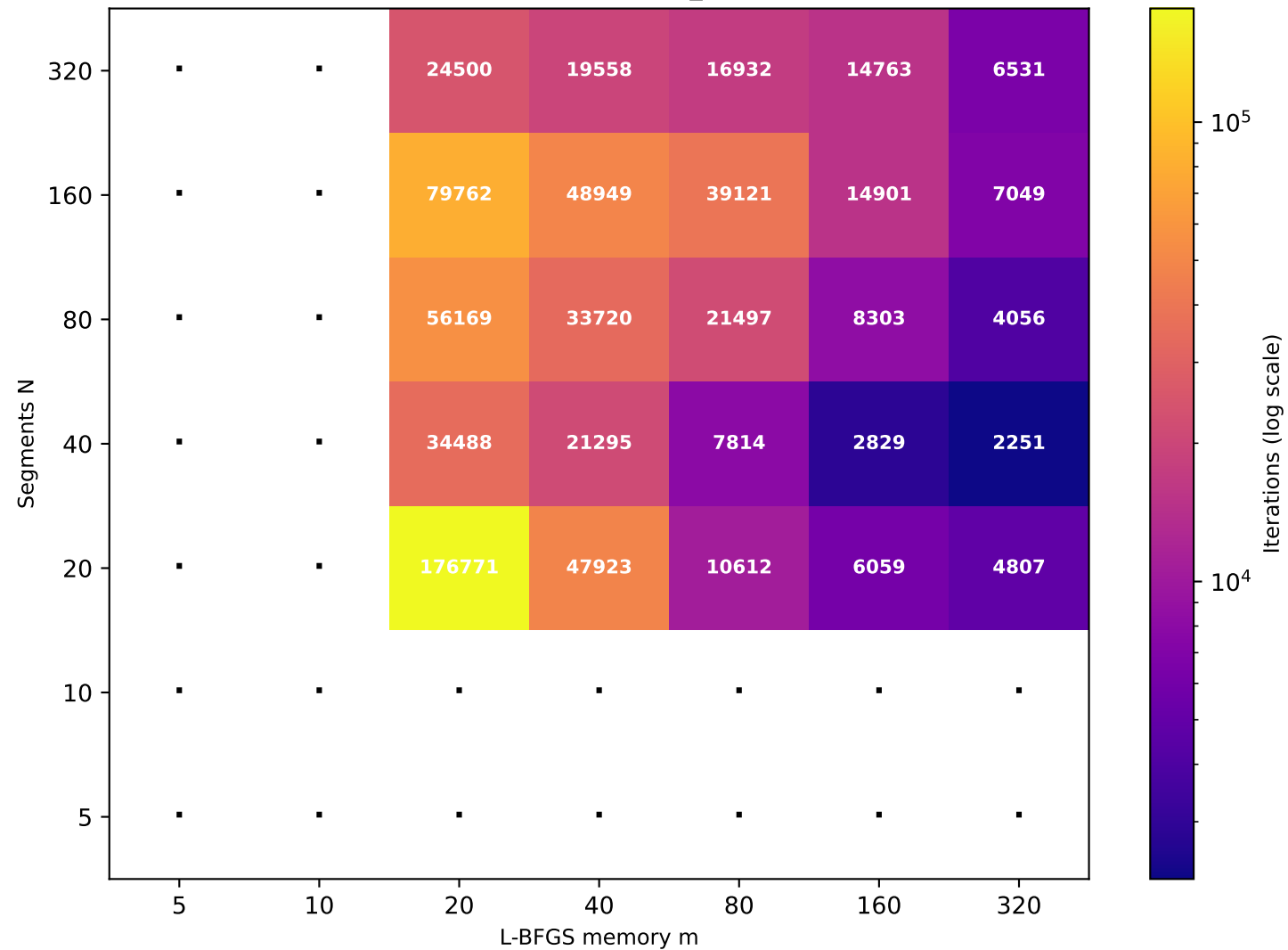
Recurrence T \approx 79.33 (target T=80 , rec_id=89) [25/49 converged]
