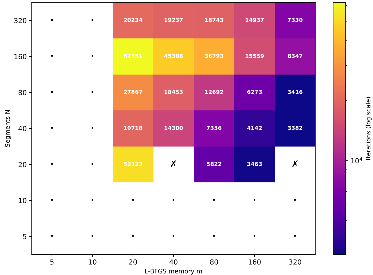
Recurrence T \approx 81.40 (target T=80 , rec_id=90) [23/49 converged]
