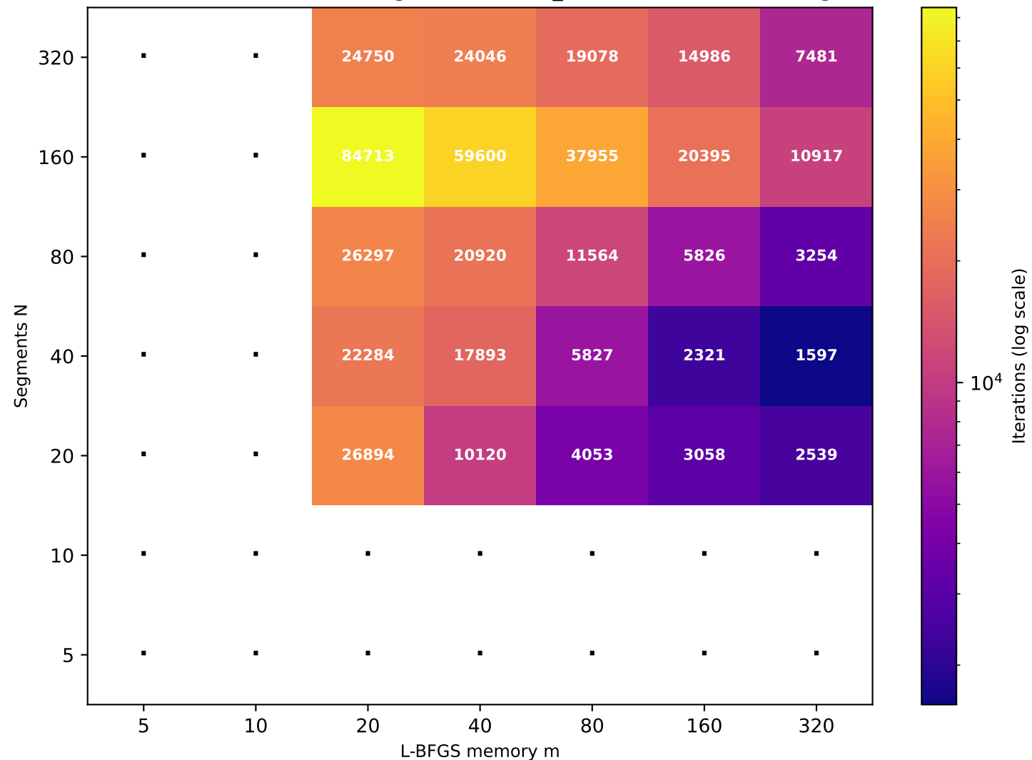
Recurrence T \approx 81.61 (target T=80 , rec_id=95) [25/49 converged]
