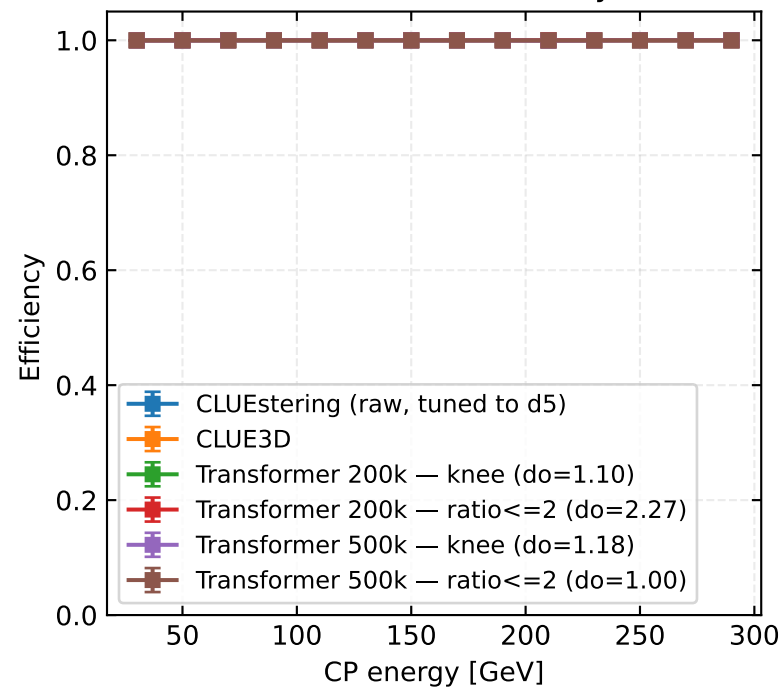
Electron: CP Efficiency
