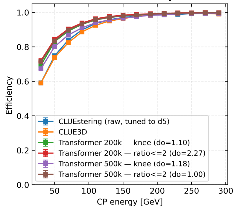
Pion: CP Efficiency
