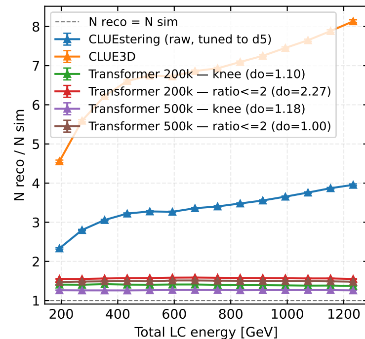
Pion: Number ratio
