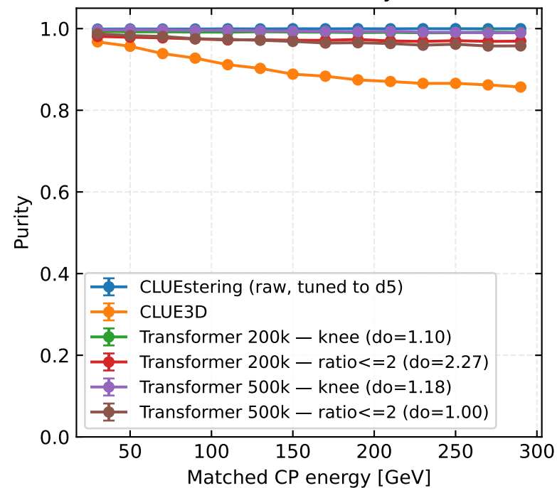
Electron: Purity
