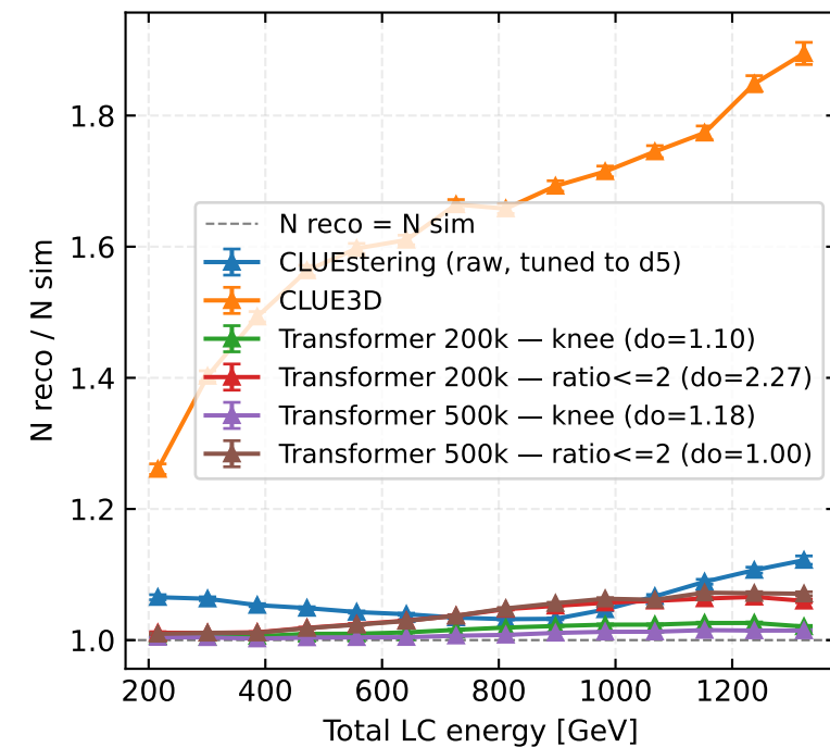
Electron: Number ratio
