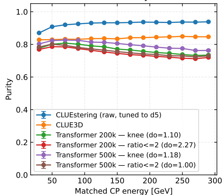
Pion: Purity
