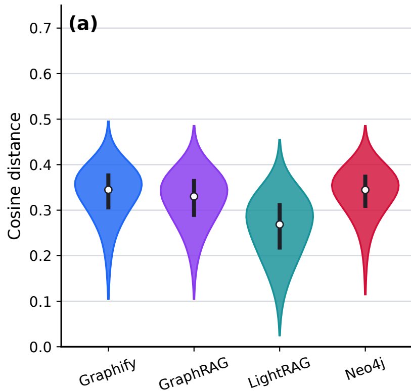
BIGS \rightarrow : documents to graph
