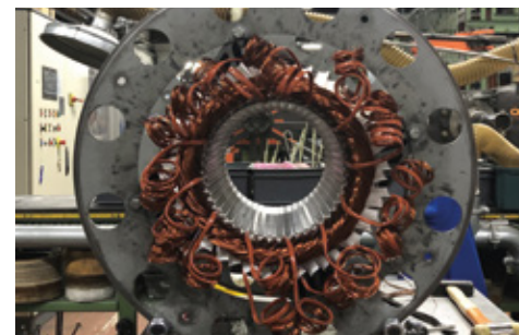
1. Dedicated winding insertion
