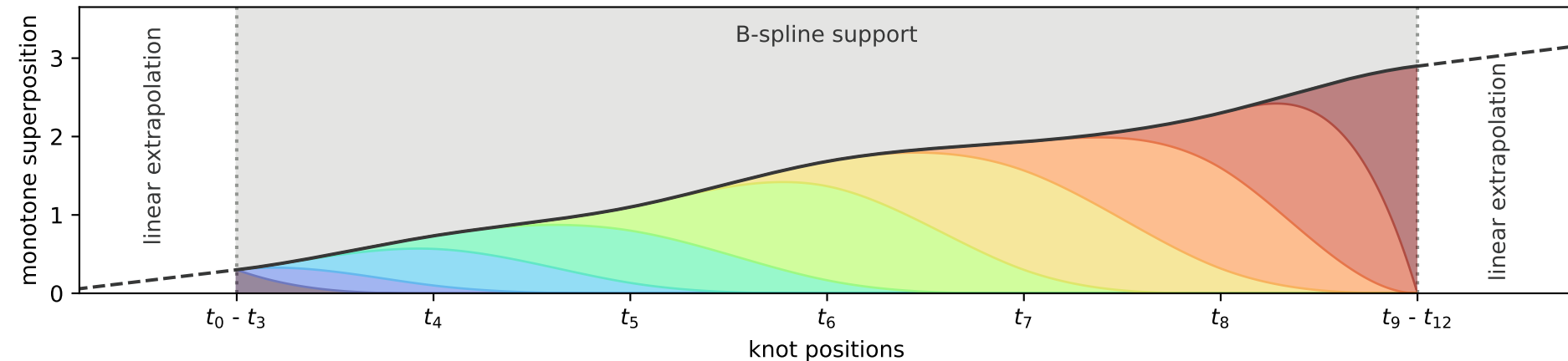
B: Resulting monotone function
