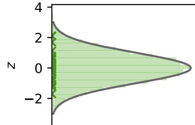
Reference distribution
