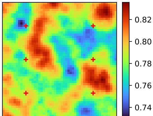
Prior std \log_{10} K (both)
