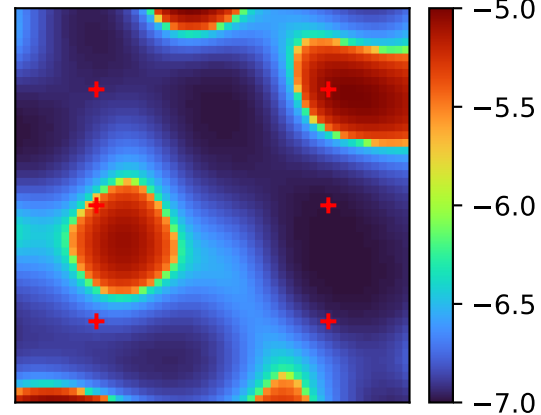
true field \log_{10} K
