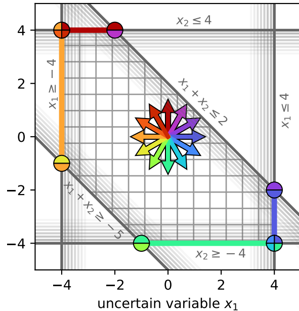
C: linear optima lie on the hull
