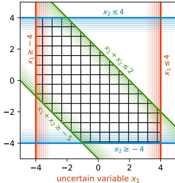
B: more constraints tighten it
