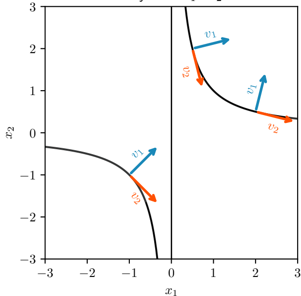
B: Nonlinear system x_1 \cdot x_2 = 1
