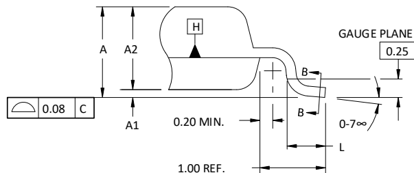
DETAIL "A"
