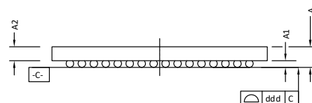
SEATING PLANE
