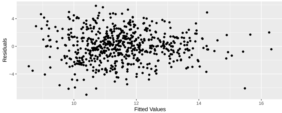
Relationship of Residuals and Fitted Values
