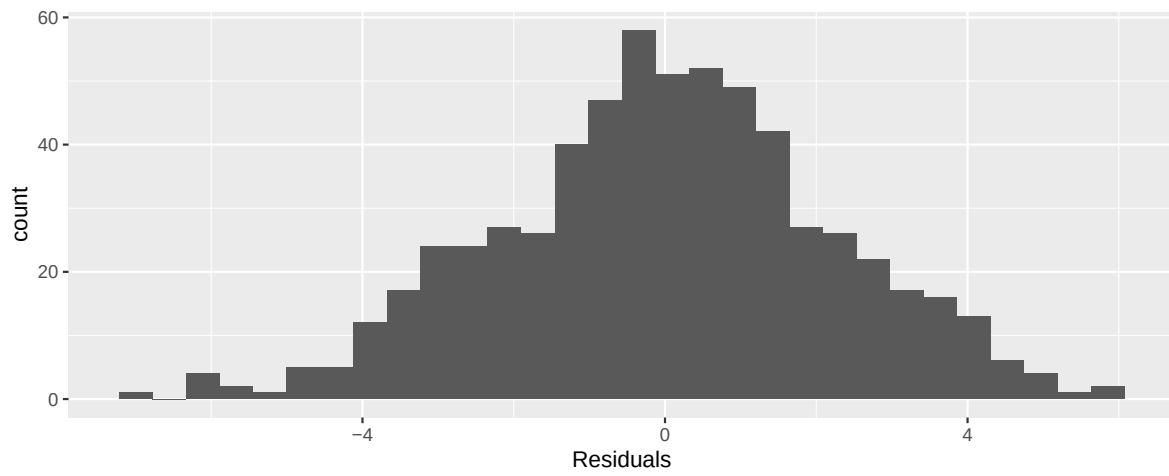
Distribution of Residual Values
