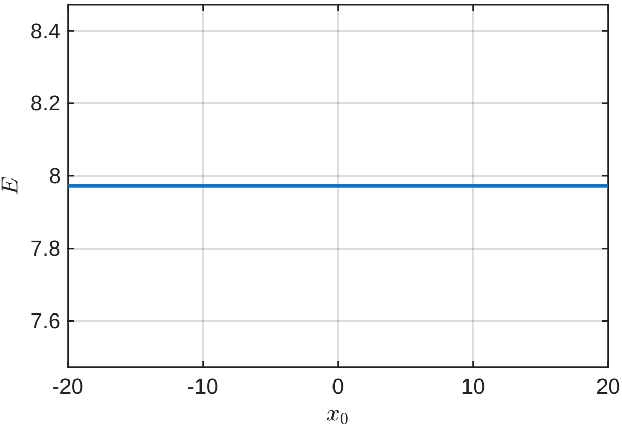
Total energy of the sine-Gordon kink vs position x_0
