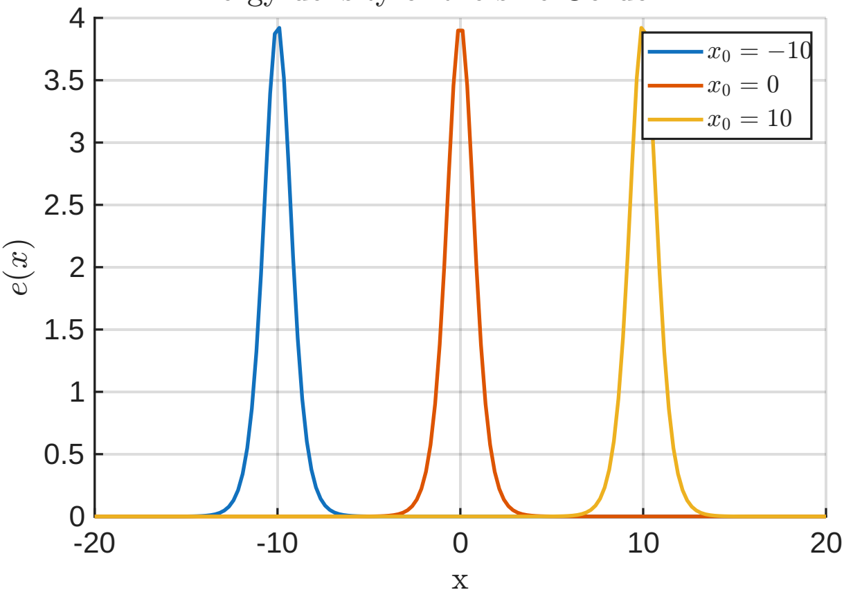
Energy density of the sine-Gordon kink
