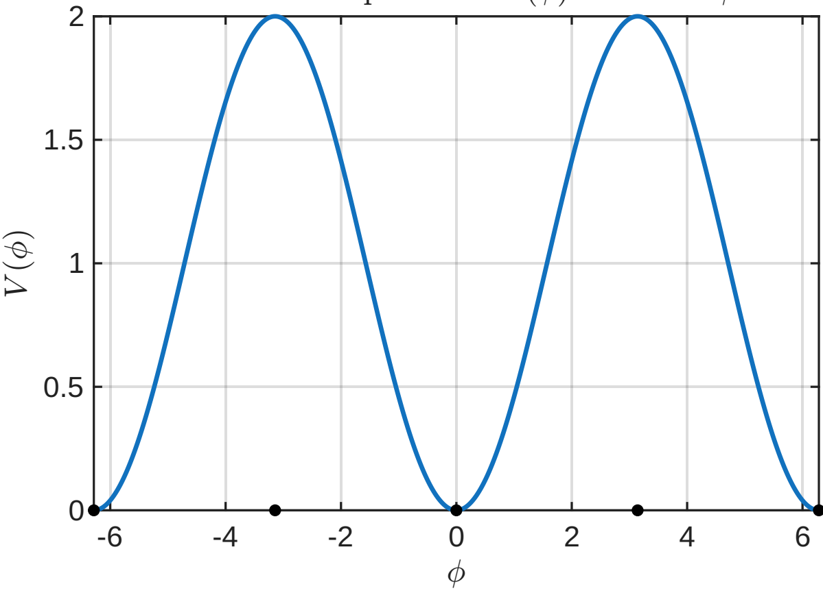
Sine-Gordon potential V(\phi) = 1 - \cos \phi
