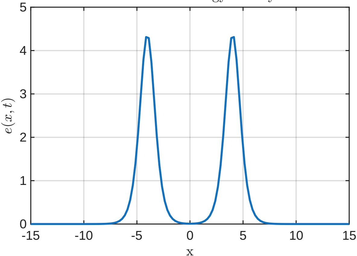
Sine-Gordon energy density
