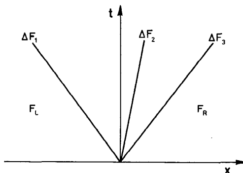
Figure 4 Diagram for computing the interface flux.
