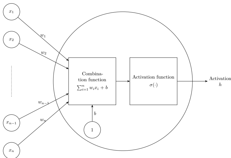
Figure 2.2: Artificial neuron.
