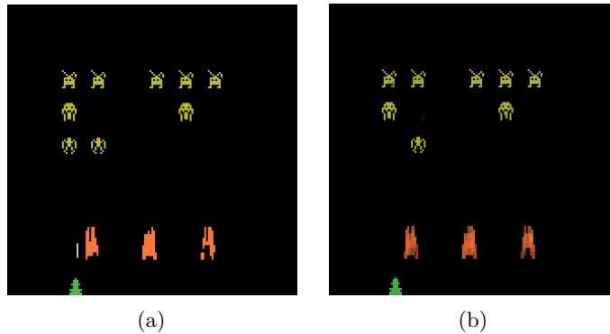
Figure 5.6: Counterfactual explanation of the agent’s behavior for the Atari game SPACE INVADERS [103]. Panel (a) shows the original observation and panel (b) the counterfactual observation produced by a generative model.
