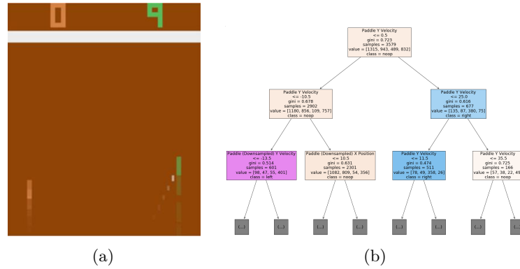
Figure 5.3: Policy approximation via an interpretable model [106].
