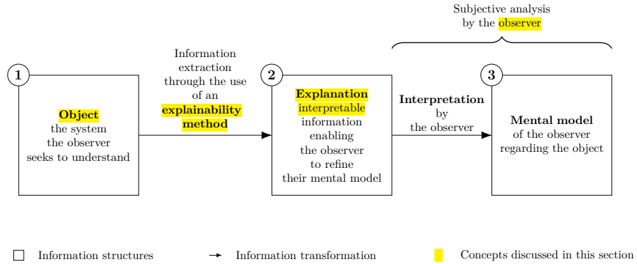
Figure 5.2: Explanation process.
