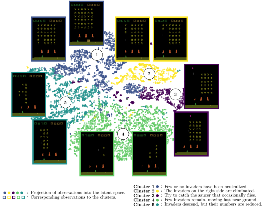
Figure 1.4: Two-dimensional projection of the LS embeddings of a surrogate policy trained on Space Invaders, together with the CAR clusters and their corresponding observations.
