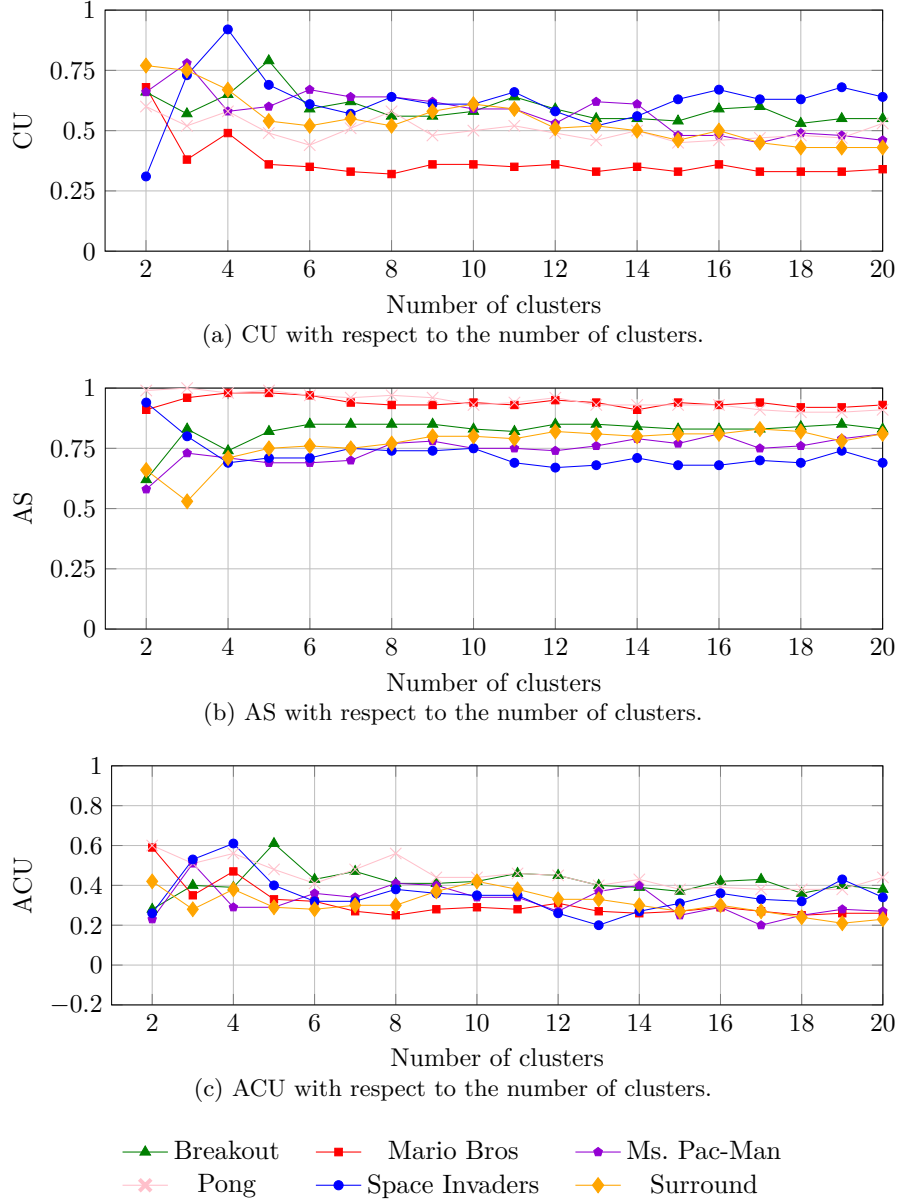
Figure 1.5: CU, AS, and ACU with respect to the number of clusters, for each of the six environments, for the layer that maximizes the average ACU in that environment.
