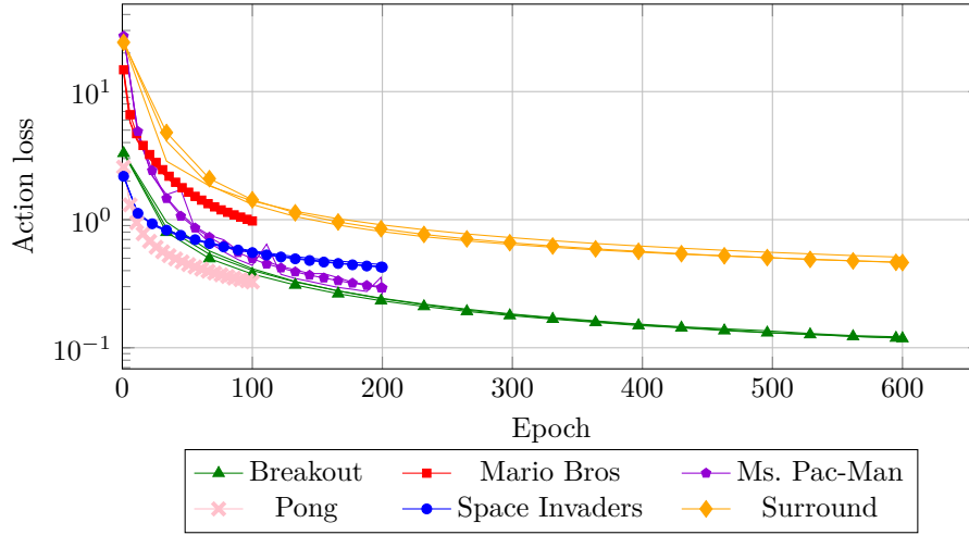
Figure 1.5: Training action loss of the surrogate policies.
