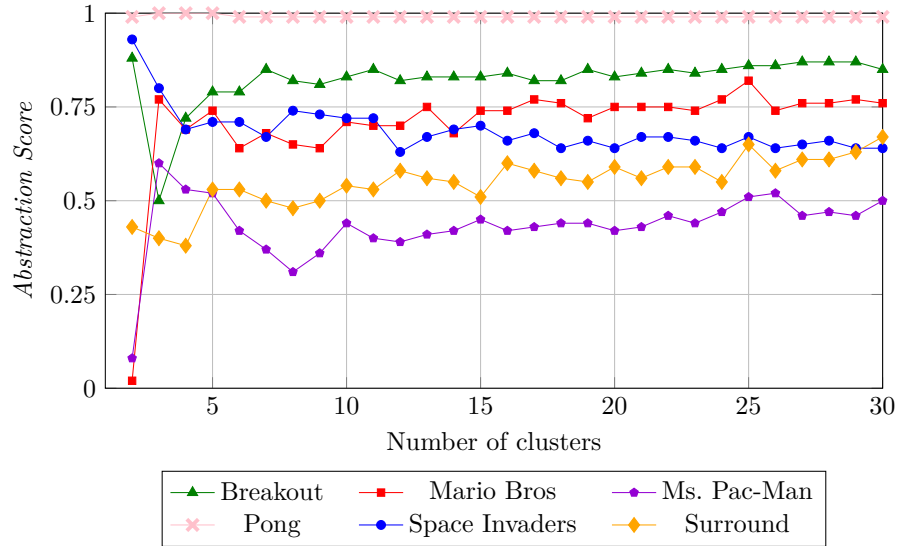
Figure 1.7: Evolution of Abstraction Score with respect to the number of clusters.
