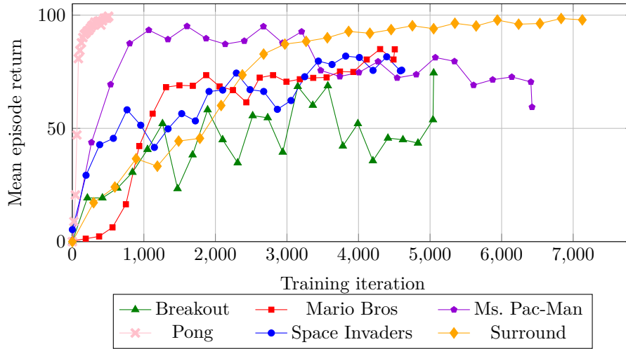
Figure 1.4: Training of the initial policies with PPO.
