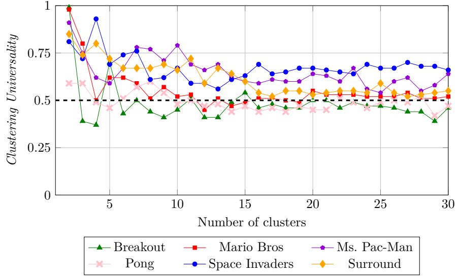
Figure 1.6: Evolution of Clustering Universality with respect to the number of clusters.
