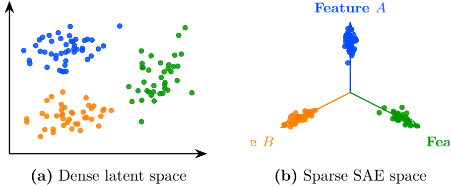
Figure 1.5: Transformation from a dense latent space to a sparse SAE-style representation. On the left (a), embeddings are entangled in the initial latent space. On the right (b), the sparse representation aligns each concept with a dedicated feature axis.
