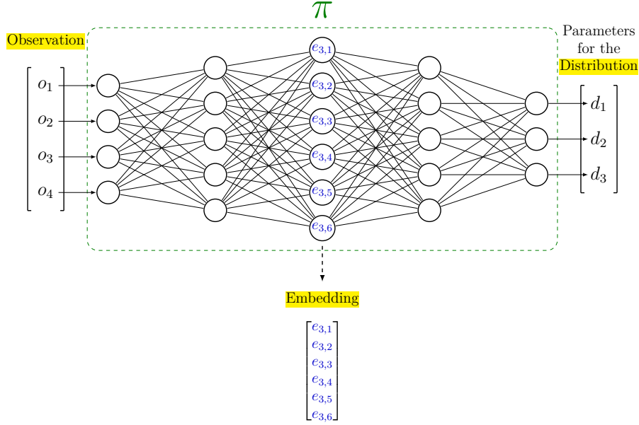
Figure 1.2: Architecture of the surrogate policy \pi . The encoder maps the observation O to the embedding, from which the decoder reconstructs the action distribution parameters.
