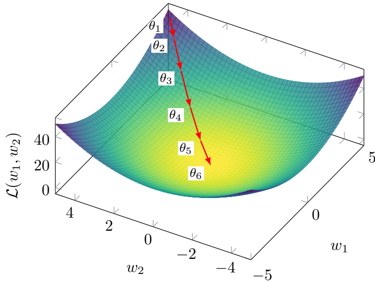
Figure 1.4: Gradient descent in a case \mathcal{L}(w_1, w_2) = w_1^2 + w_2^2 .
