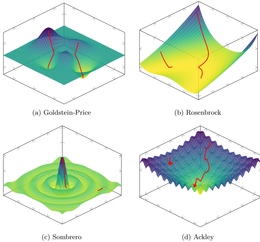
Figure 1.5: Comparison of loss surfaces and gradient descent trajectories.
