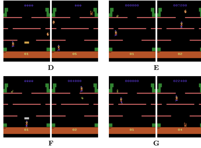
Figure 1.10: Clusters D–G identified by CAR in the Mario Bros environment (layer 8b, K = 4 ).
