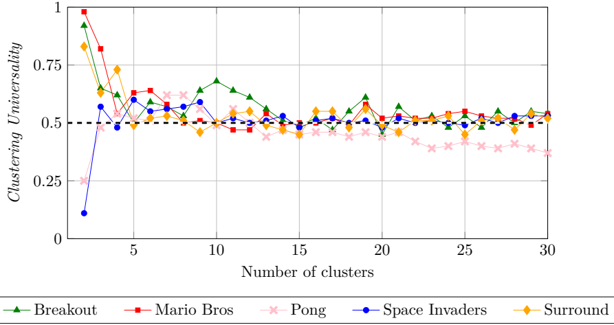
Figure 5.4: Evolution of Clustering Universality with respect to the number of clusters, for each of the five Atari environments.
