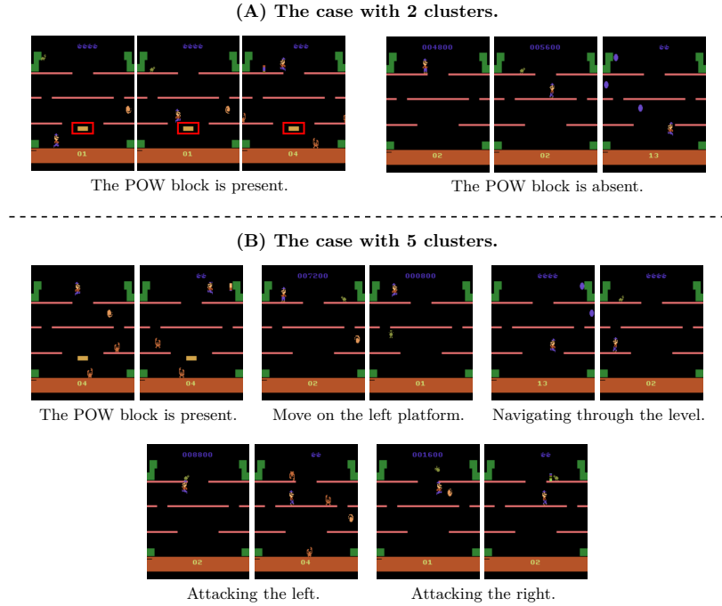
Figure 5.5: Effect of the number of clusters on the groupings identified by CAR in the Mario Bros environment.
