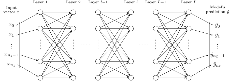
Figure 1.2: Illustration of a Multilayer Perceptron Architecture.
