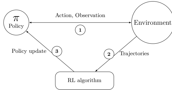
Figure 1.4: The three steps of a reinforcement learning iteration.
