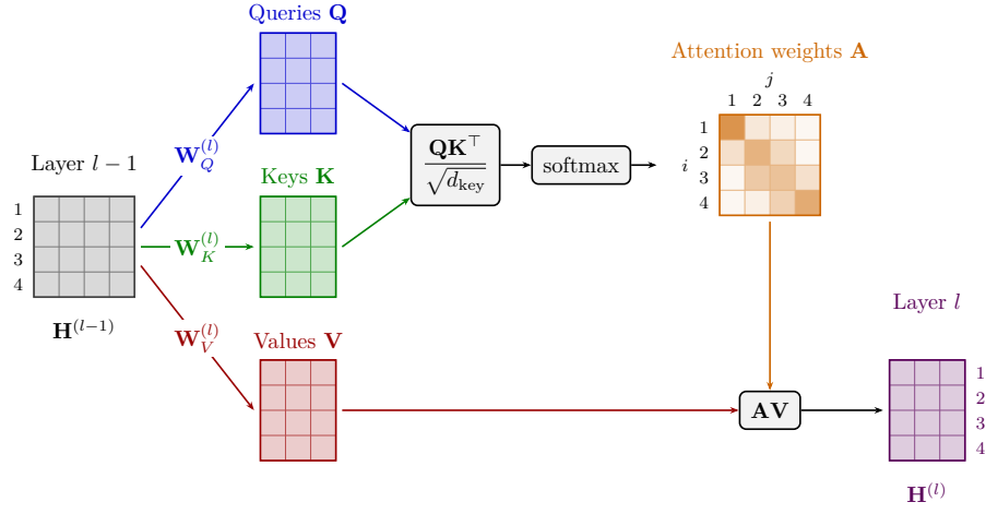
Figure 2.8: Attention mechanism.
