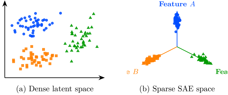
Figure 3.7: Transformation from a dense LS (a) to a sparse SAE representation (b).
