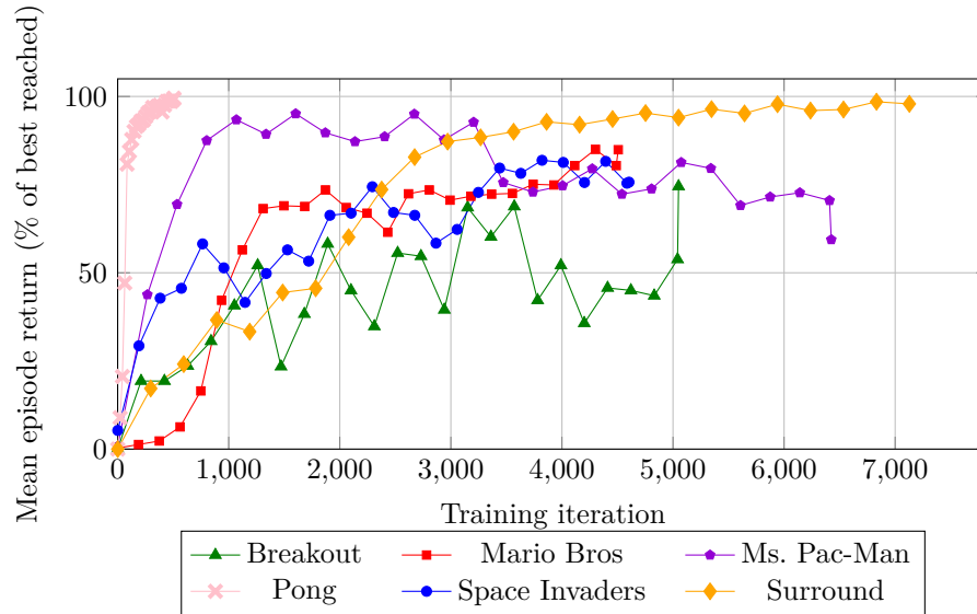
Figure 1.4: Training of the initial policies with PPO.
