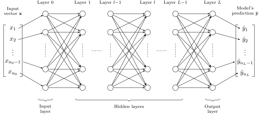
Figure 2.3: MLP architecture.
