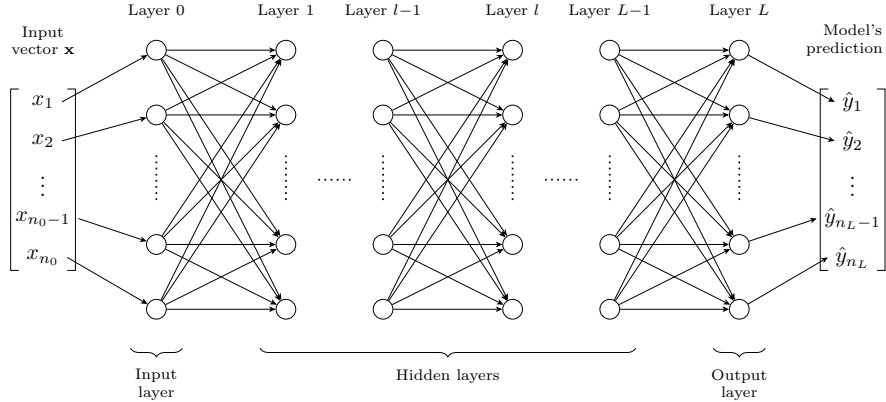
Figure 2.3: MLP architecture.
