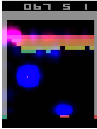
Figure 1.2: Perturbation-based heatmap for the Atari game “Breakout” [Greydanus et al., 2018]. Highlighted areas correspond to the most influential regions for the policy function’s decision.
