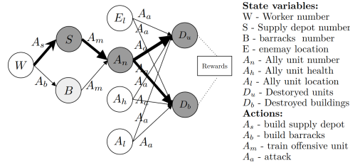
Figure 1.5: Agent-environment interaction model for the video game StarCraft II [Madumal et al., 2020]. Nodes represent random variables, and edges represent causal relationships between them.
