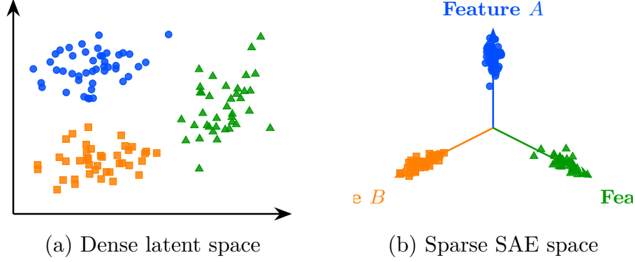
Figure 3.7: Transformation from a dense latent space (a) to a sparse SAE representation (b).
