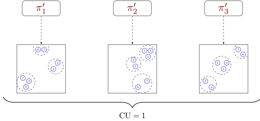
Figure 6.4: Illustration of CU in the ideal case where projections of the same observations are grouped within the same clusters across all surrogate policies.
