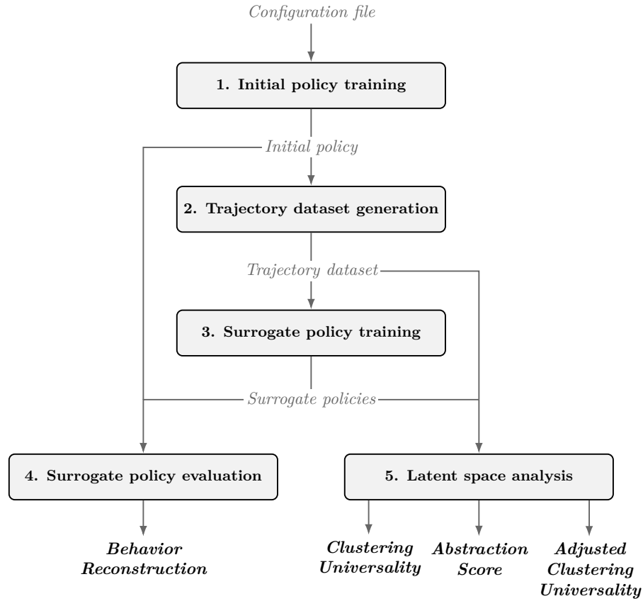
Figure 7.1: The CAR pipeline.
