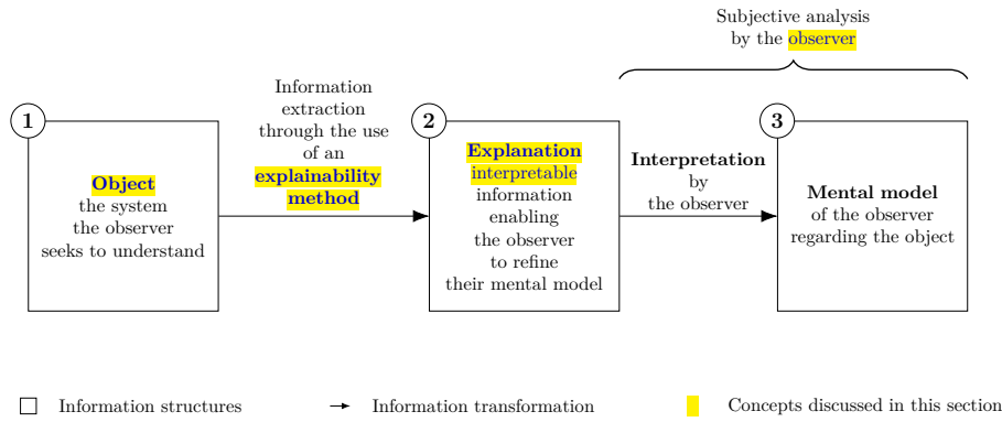
Figure 5.2: Explanation process.
