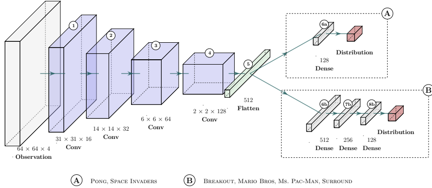
Figure 7.3: Architecture of the surrogate policies.
