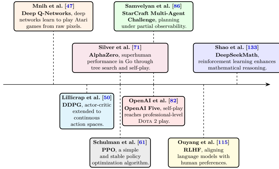
Figure 4.2: Evolution of deep reinforcement learning.
