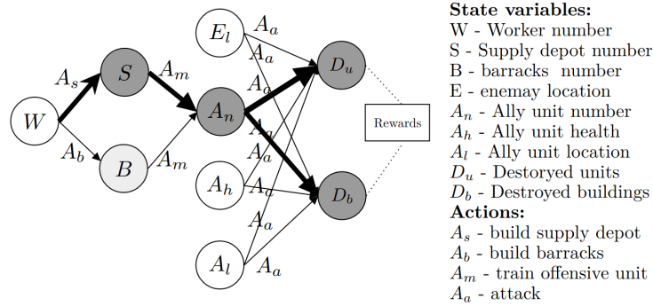
Figure 5.8: Agent-environment interaction model for the video game STAR-CRAFT II [95].
