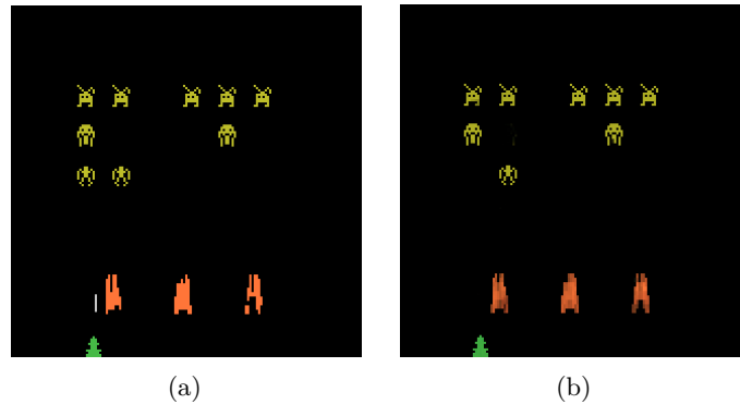
Figure 5.6: Counterfactual explanation of the agent’s behavior for the Atari game SPACE INVADERS [108]. Panel (a) shows the original observation and panel (b) the counterfactual observation produced by a generative model.
