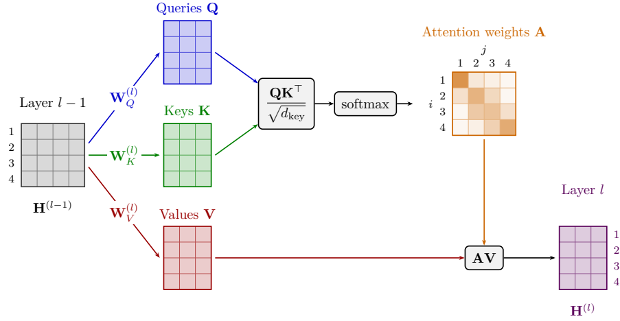
Figure 2.8: Attention mechanism.
