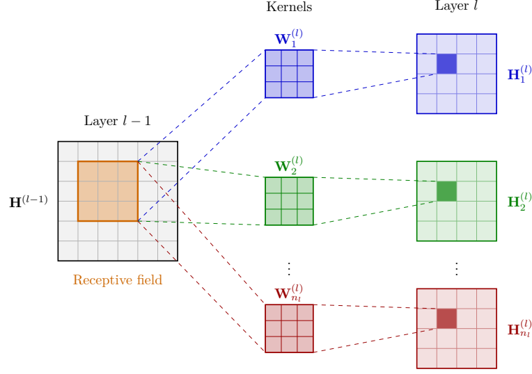
Figure 2.7: Convolutional layer.
