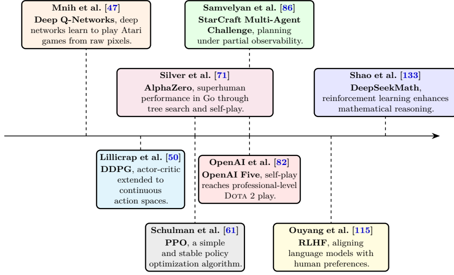
Figure 4.2: Evolution of deep RL.
