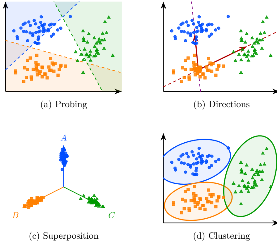
Figure 3.11: Overview of the four LS analysis methods studied in this chapter, applied to the same point cloud.
