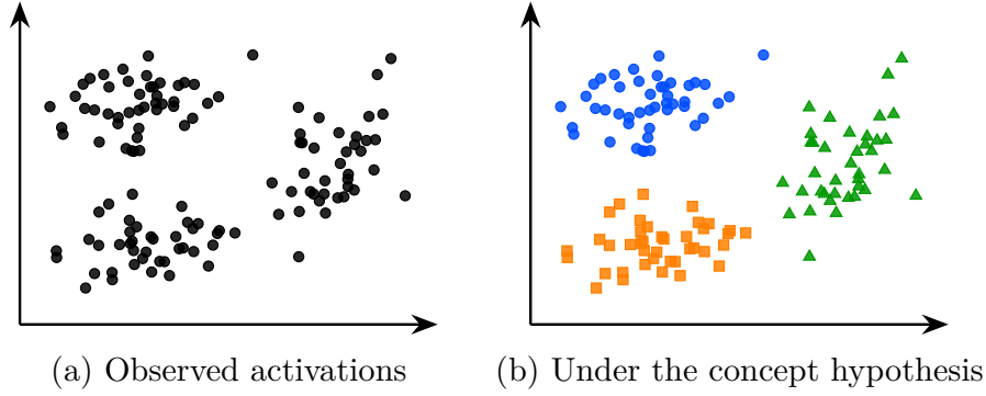
Figure 3.1: The same LS activations seen without (a) and under (b) the Concept Hypothesis (Hypothesis 1).
