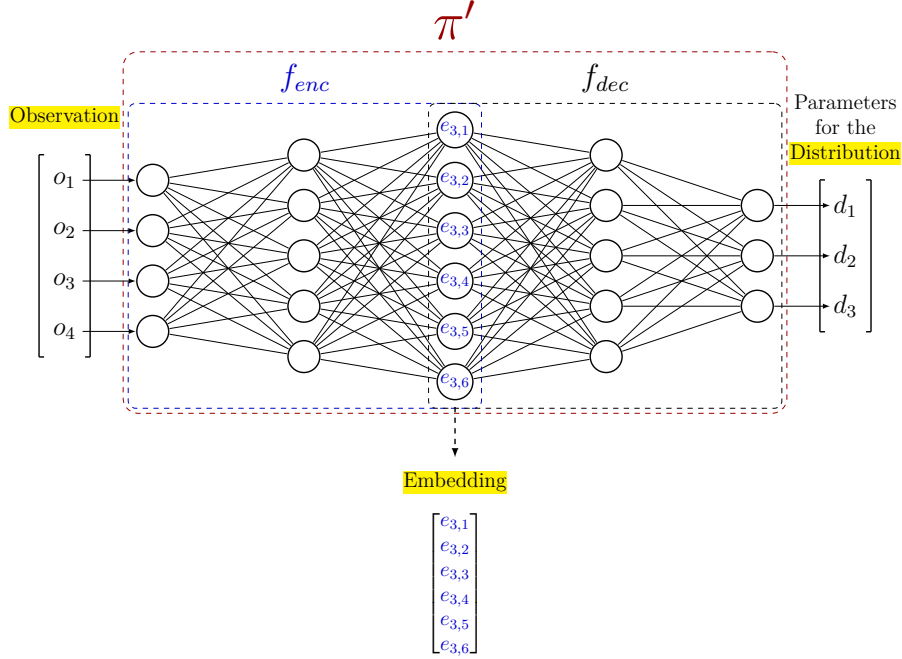
Figure 6.2: Example of a surrogate policy architecture \pi' .
