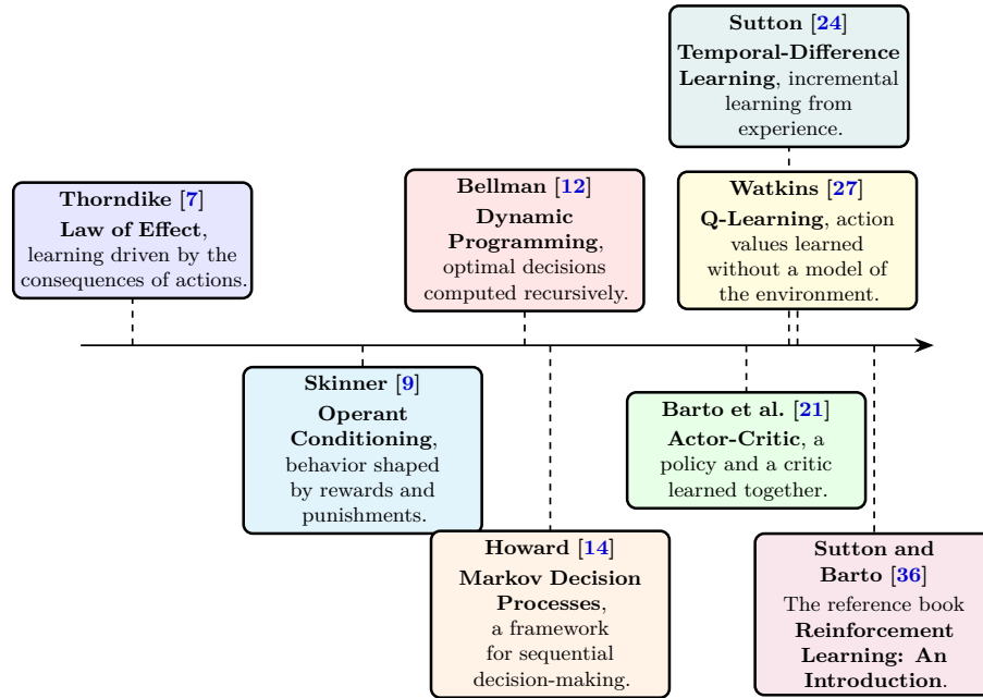
Figure 4.1: Evolution of reinforcement learning prior to its fusion with deep learning.
