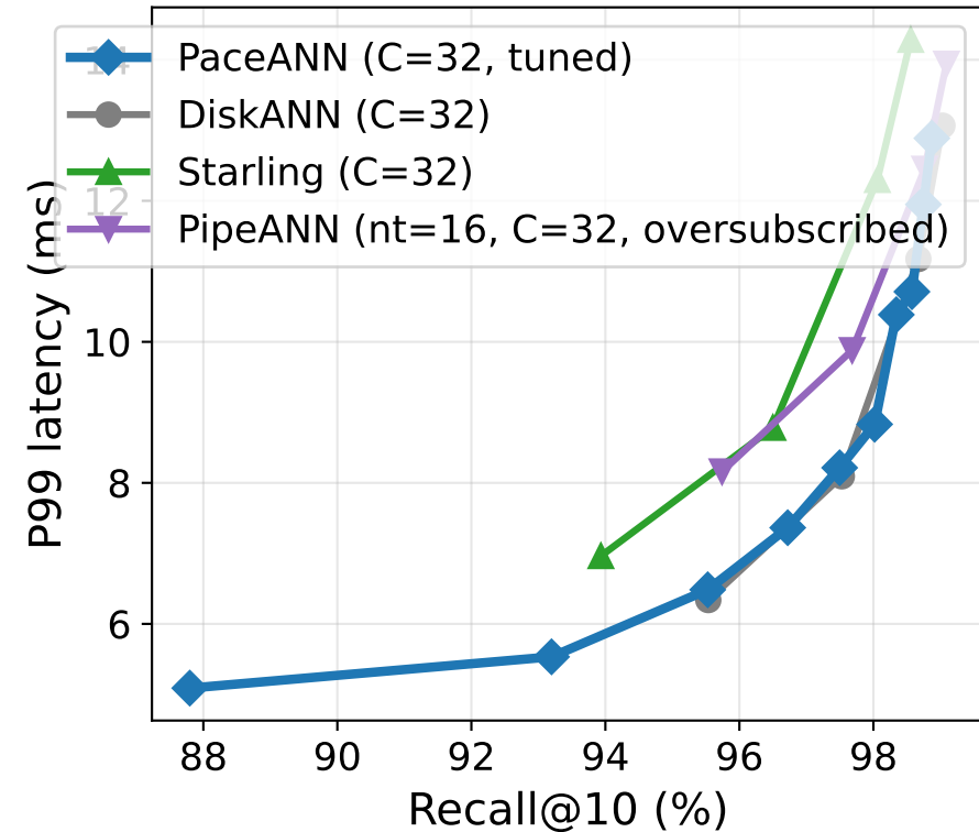
DEEP100M
