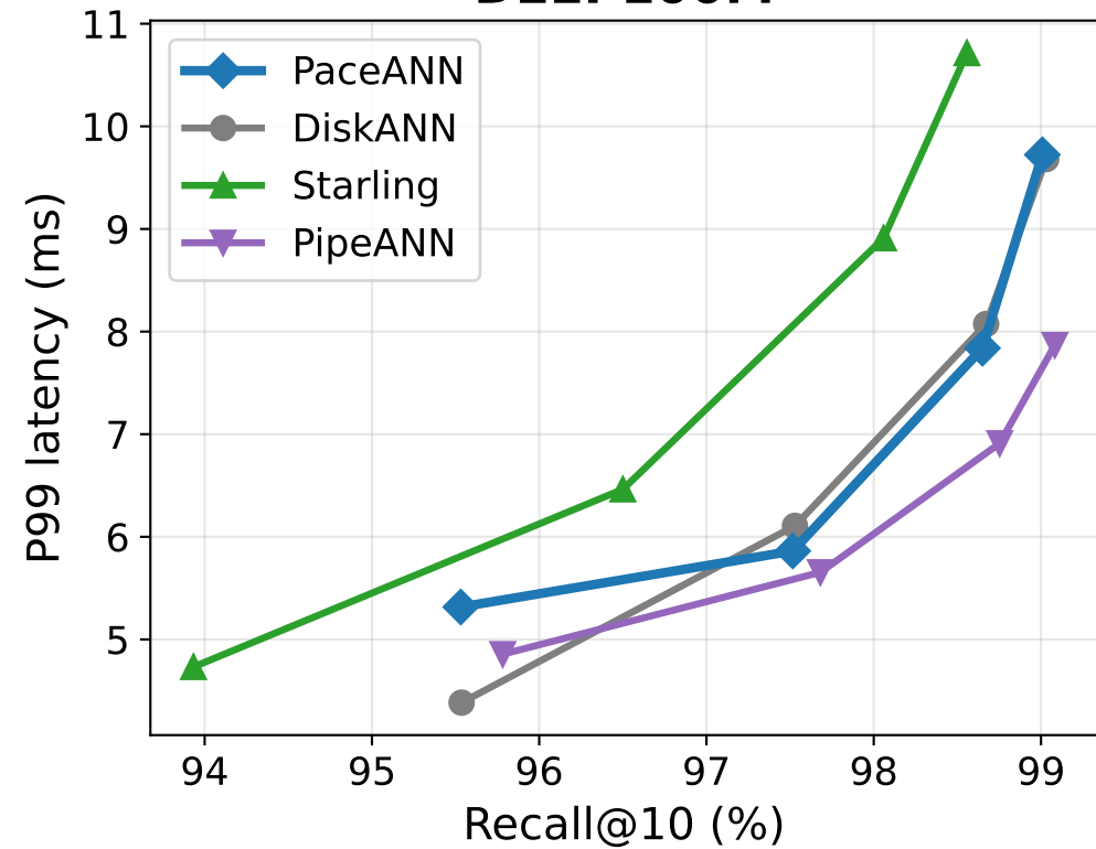
DEEP100M
