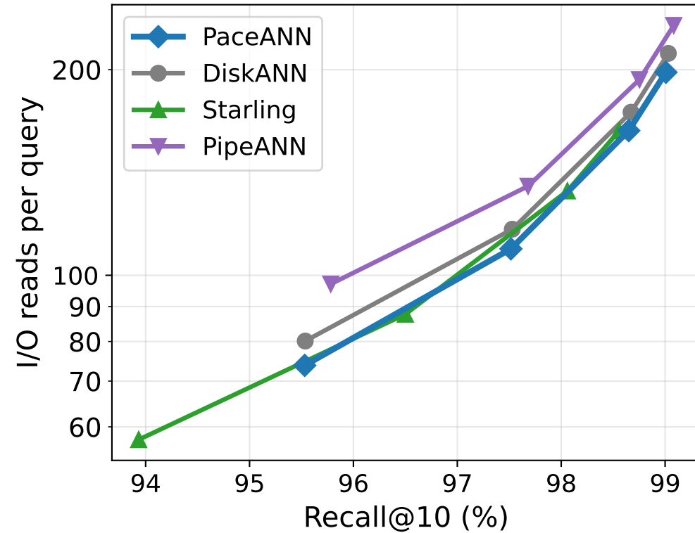
DEEP100M
