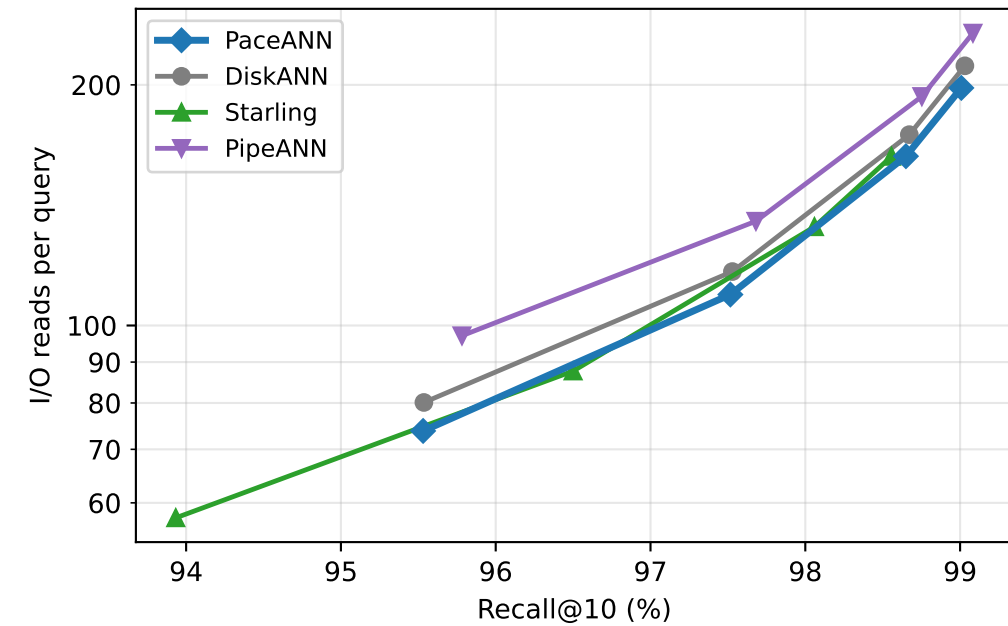
DEEP100M
