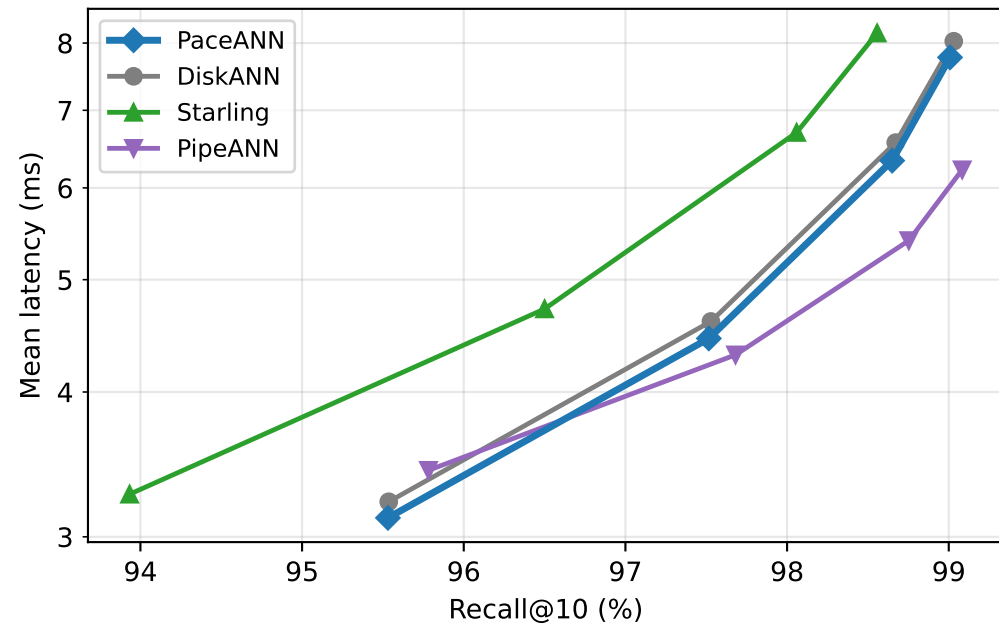
DEEP100M
