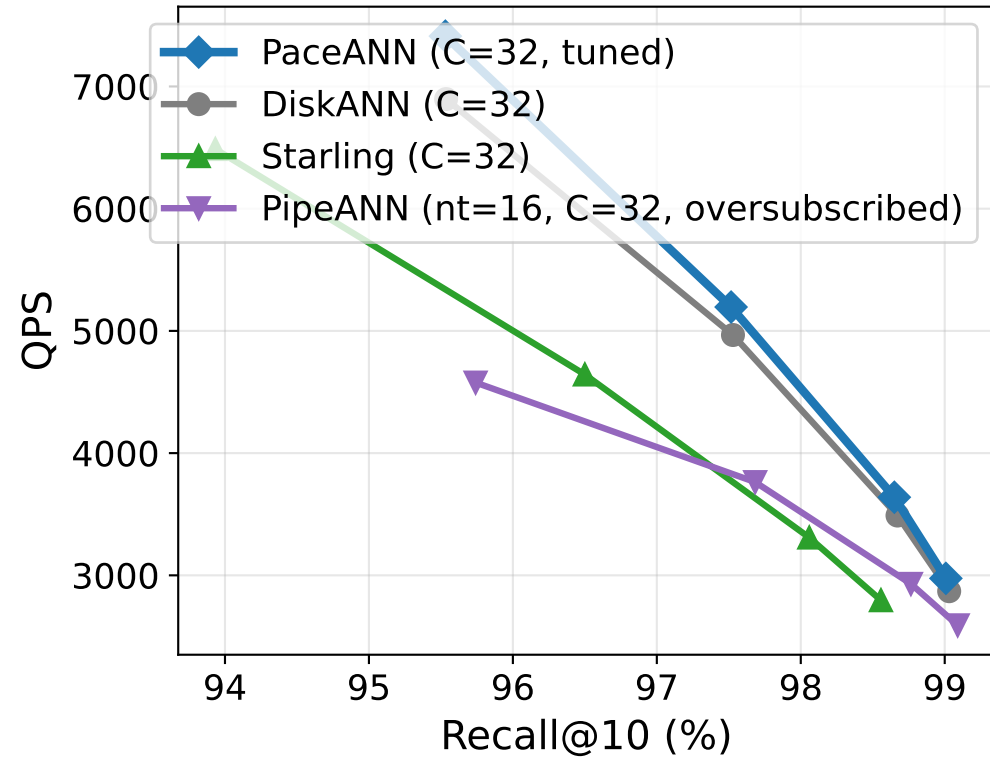
DEEP100M
