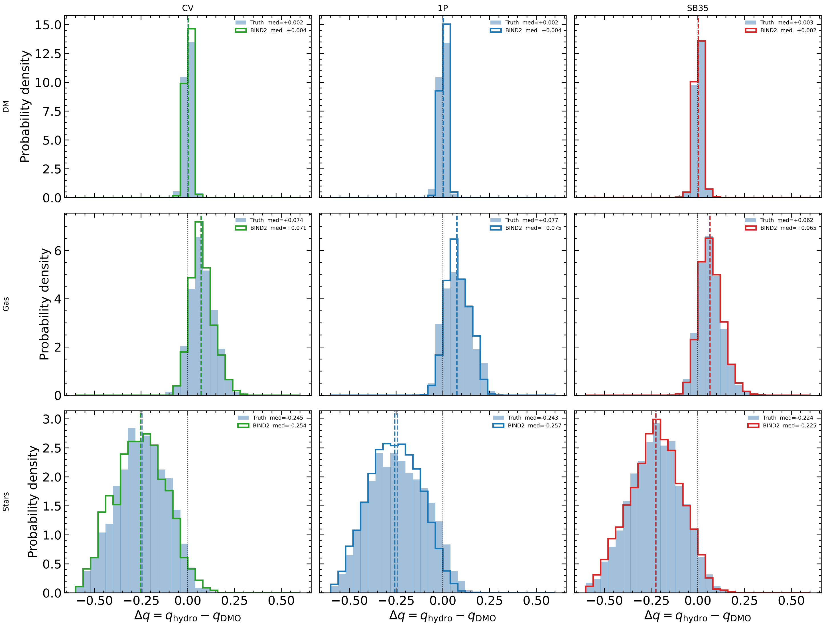
Baryonic rounding \Delta q = q_{\text{hydro}} - q_{\text{DMO}} (positive = rounder under baryons)
