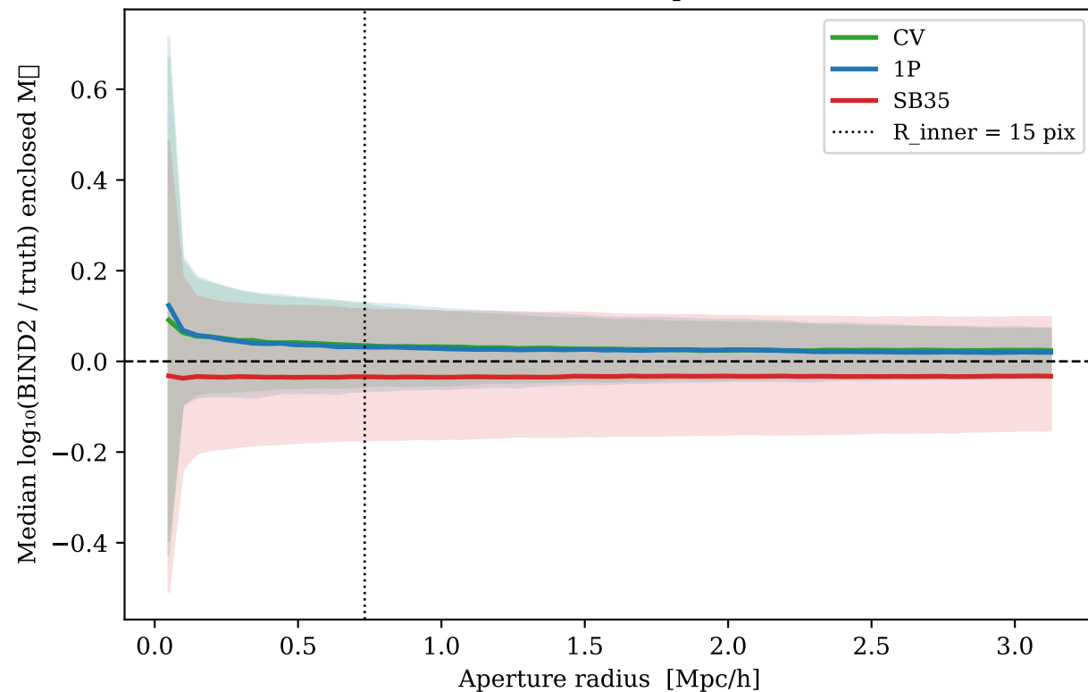
Cumulative stellar mass bias vs aperture (shaded = 16-84th percentile)
