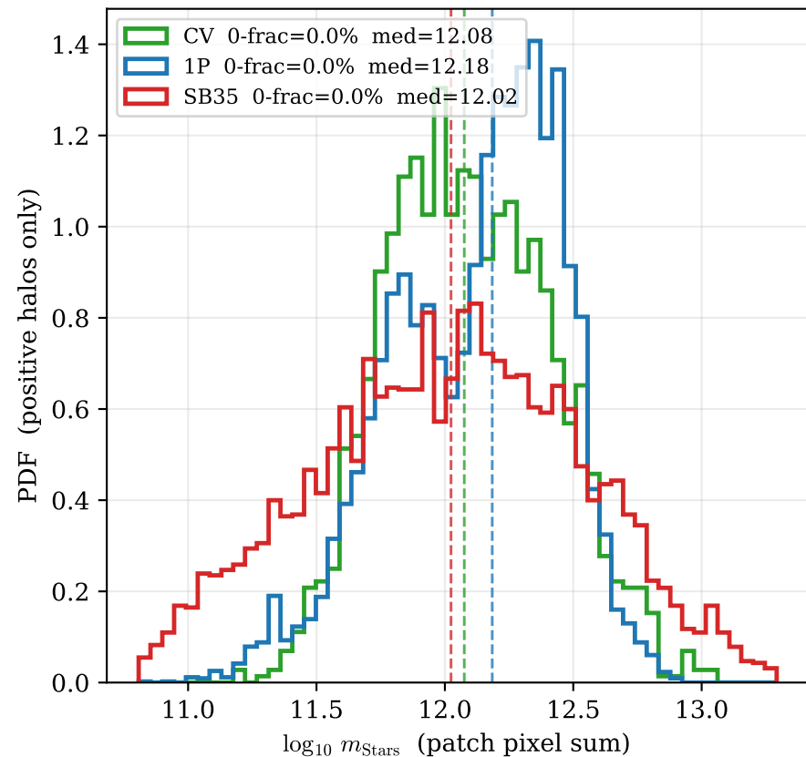
Truth stellar mass per halo patch
