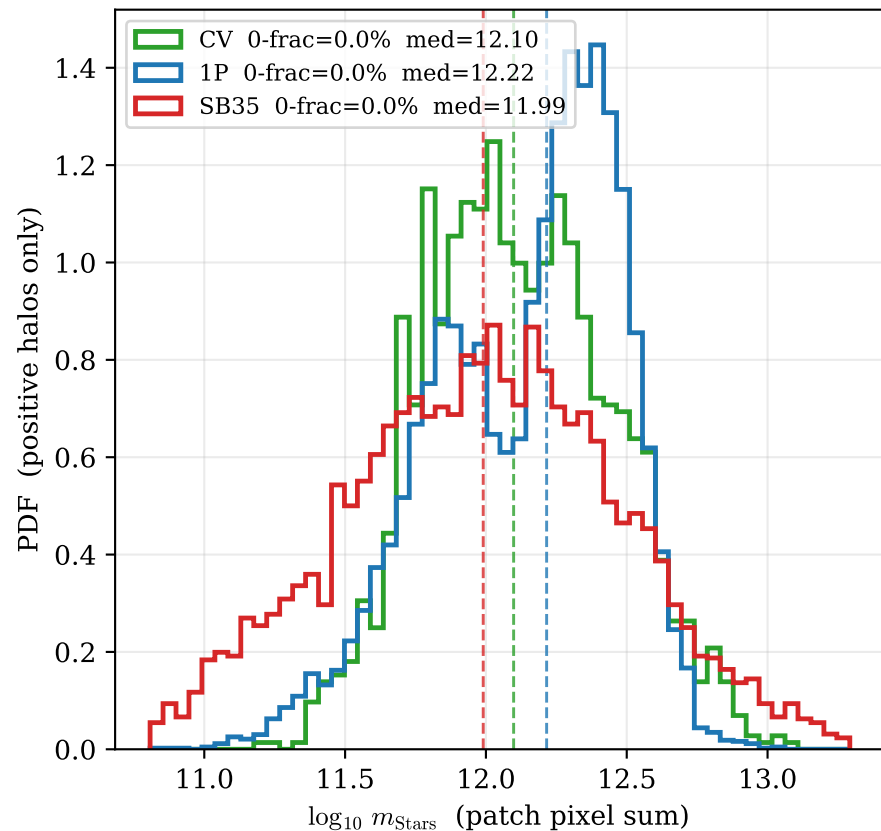
Generated stellar mass per halo patch
