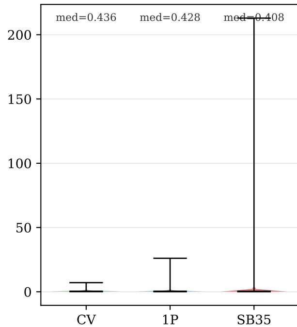
Stars
