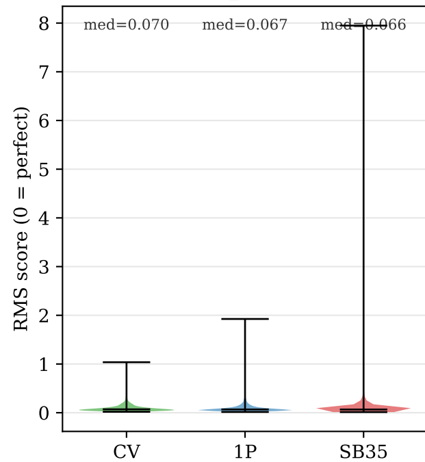
DM_hydro
