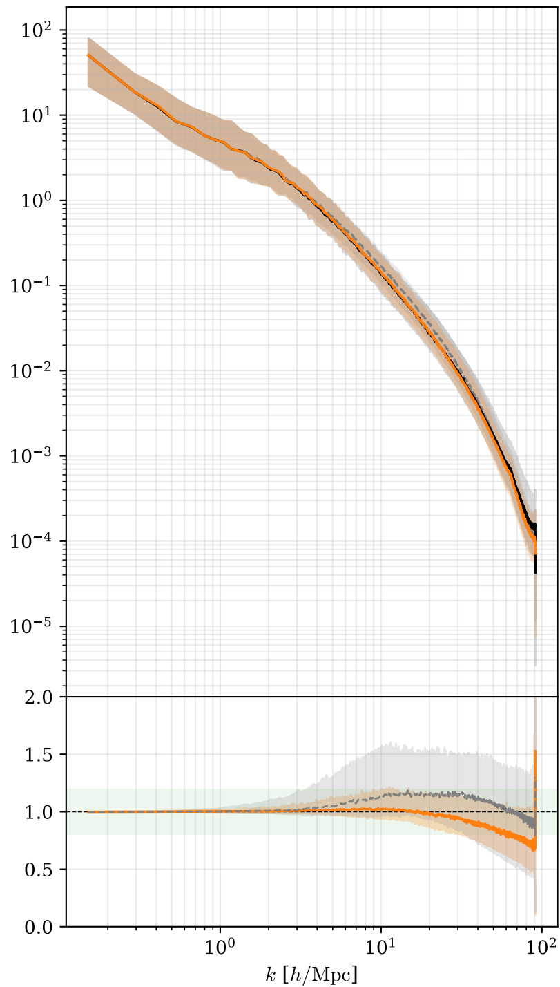
SB35 total-field P(k) (n=102 sims)
