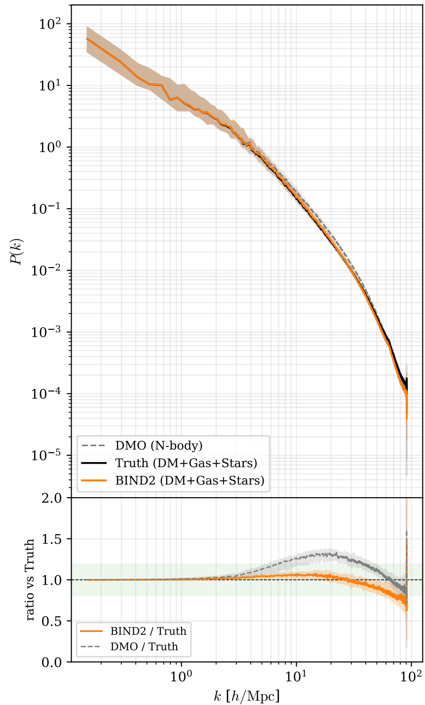
CV total-field P(k) (n=27 sims)
