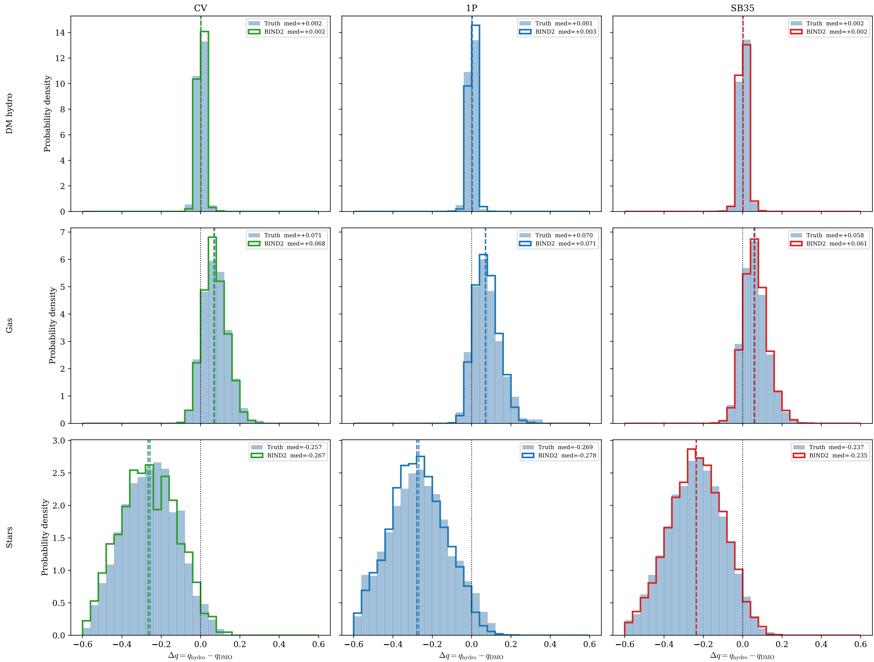
Baryonic rounding \Delta q = q_{\text{hydro}} - q_{\text{DMO}} (positive = rounder under baryons)
