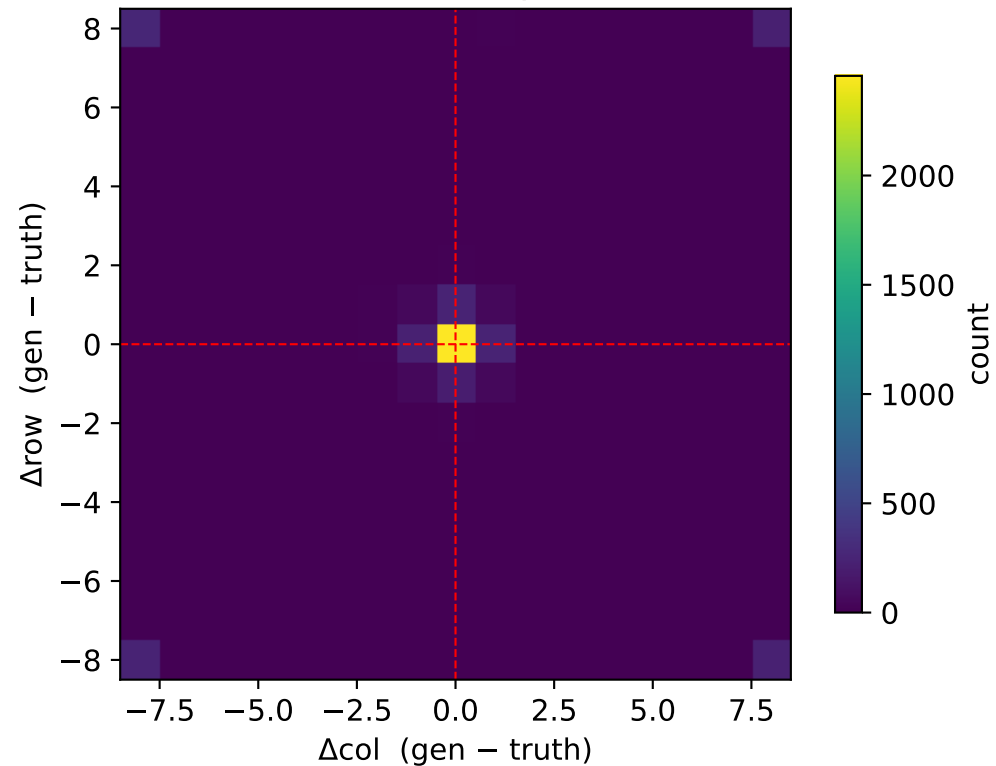
P4: BCG offset heatmap — Stars exact=49.1% \leq 1\text{px} =71.3%
